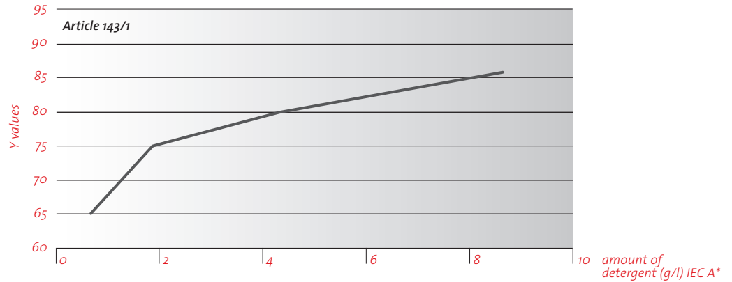
Influence of amount of detergent, 60 °C
