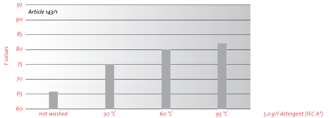
Influence of washing temperature
